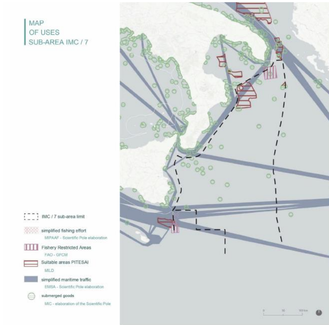
Figure 39. Summary map of the main uses present in the IMC/7 Sub-area Ionian-Central Mediterranean Continental Shelf
